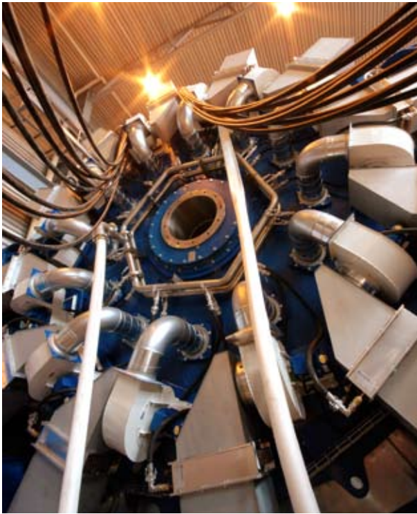
The Switch Permanent Magnet Generator: up to 20% more energy per year.
